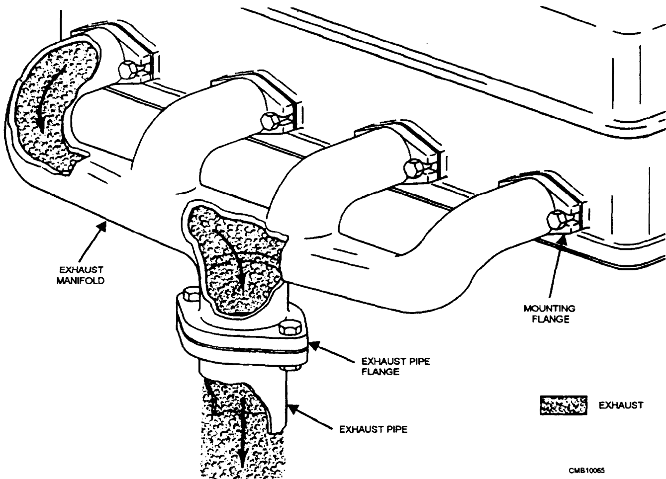
Figure 3-14.—Exhaust manifold.
