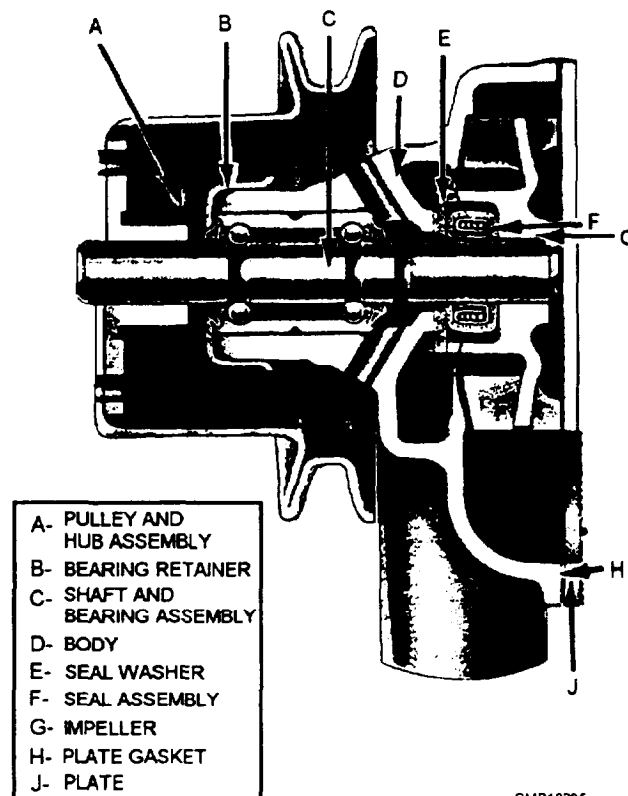
Figure 6-7.—Water pump.
